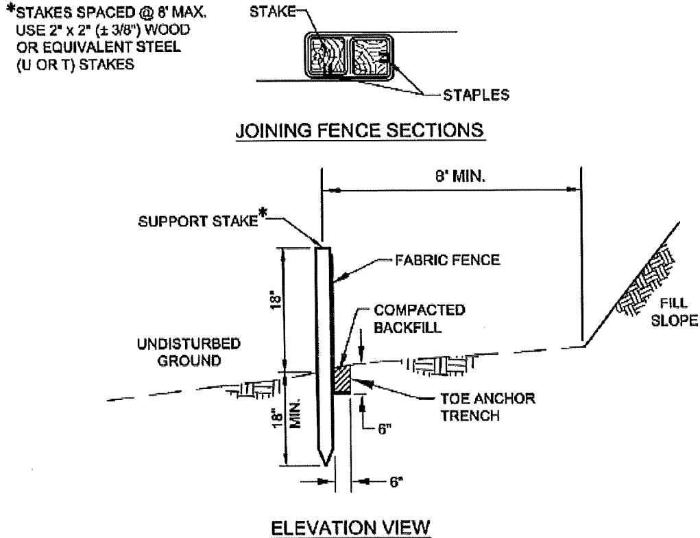
Figure 7. Standard Construction Detail for Silt Fence
