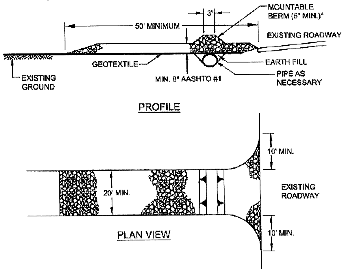
Figure 11. Standard Construction Detail for Rock Construction Entrance
