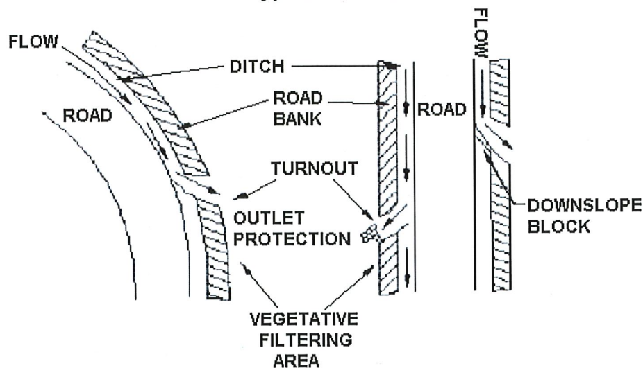
FIGURE 3.3 Typical Turnout
