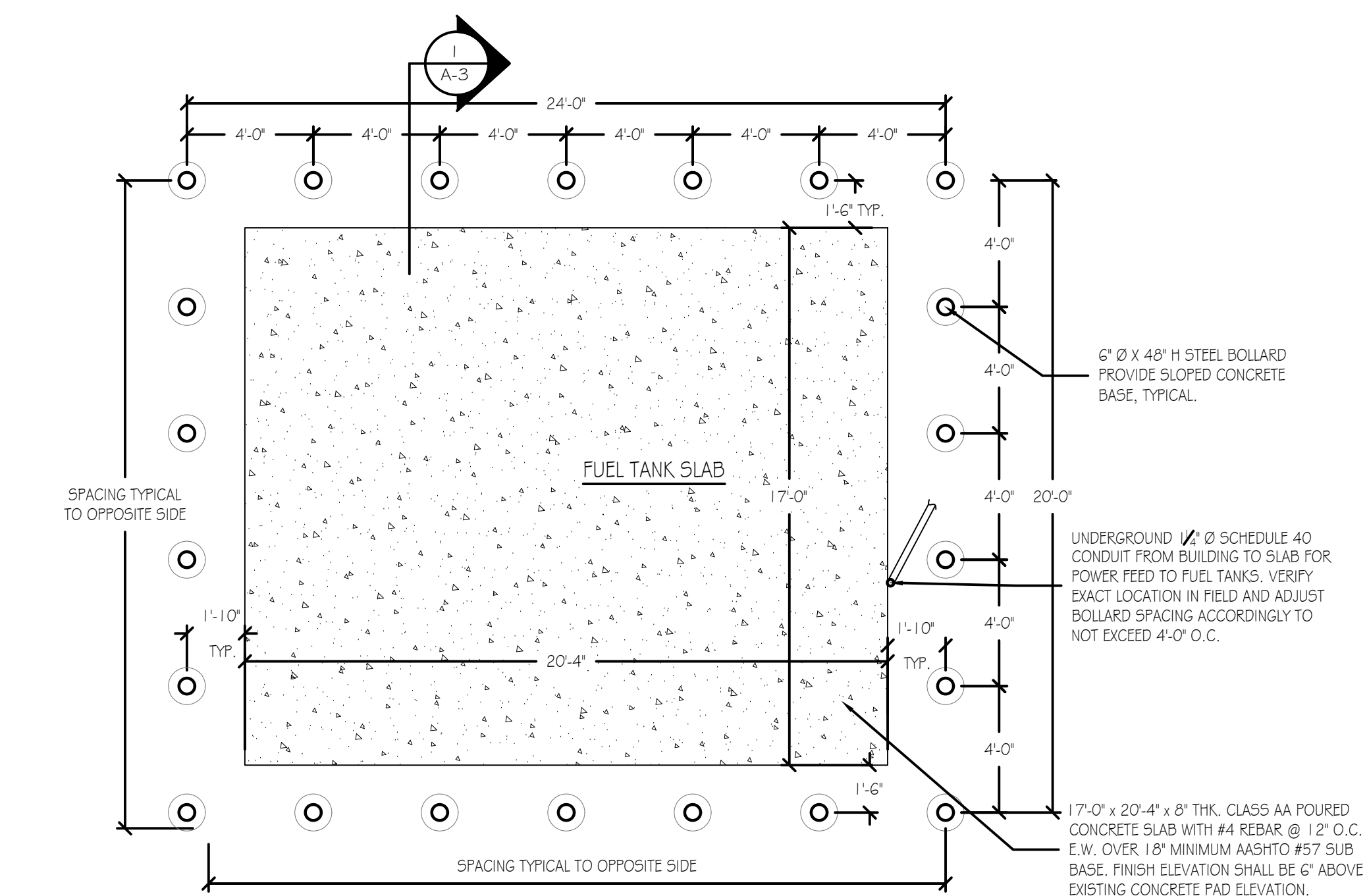
FUEL TANK SLAB PLAN SCALE: 1/4" = 1'-0"
