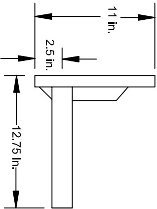
CENTER RECEIVER, WALLACE FORGE PART NUMBER RE8511
