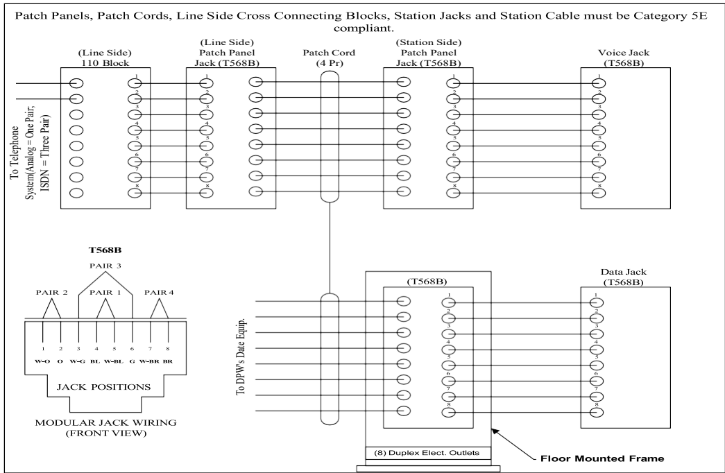
Wiring Diagram
