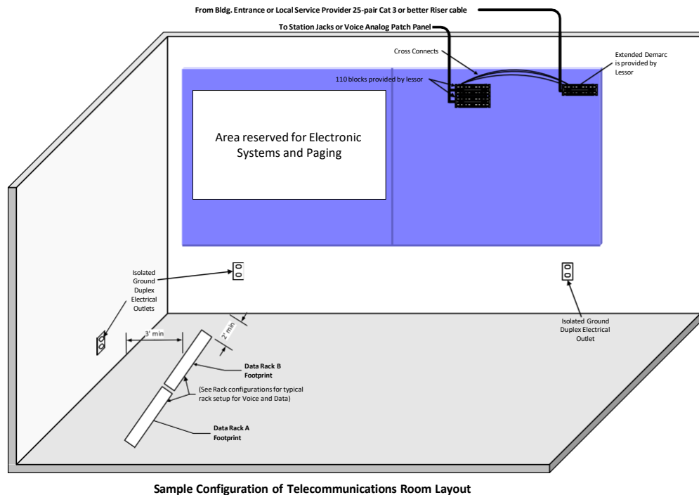
Sample Configuration of Telecommunications Room Layout
