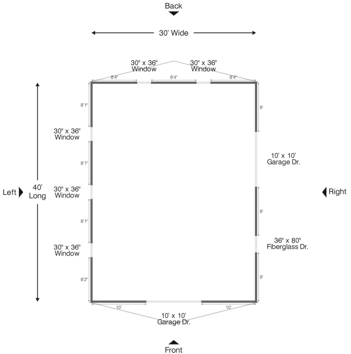
Floor Plan
