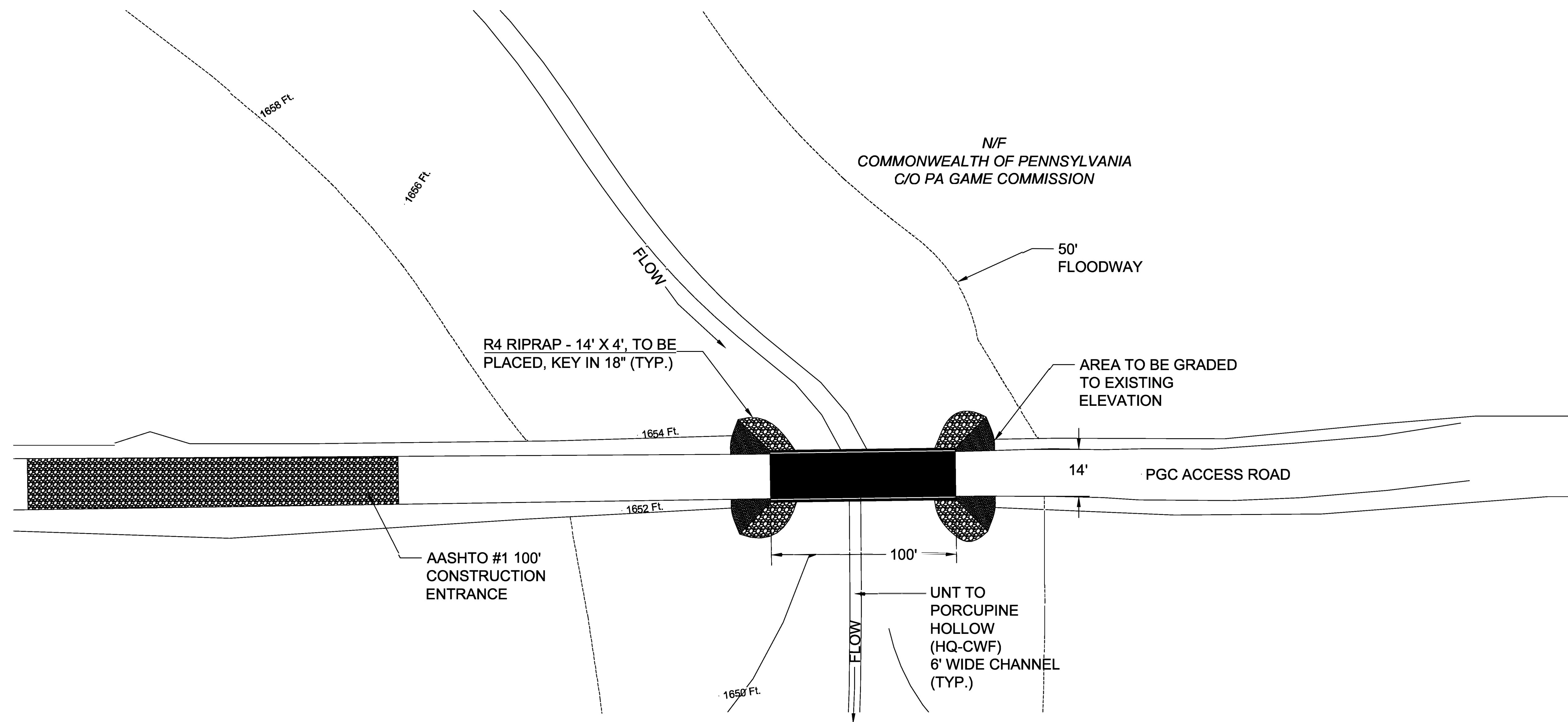
PROPOSED BRIDGE NTS
